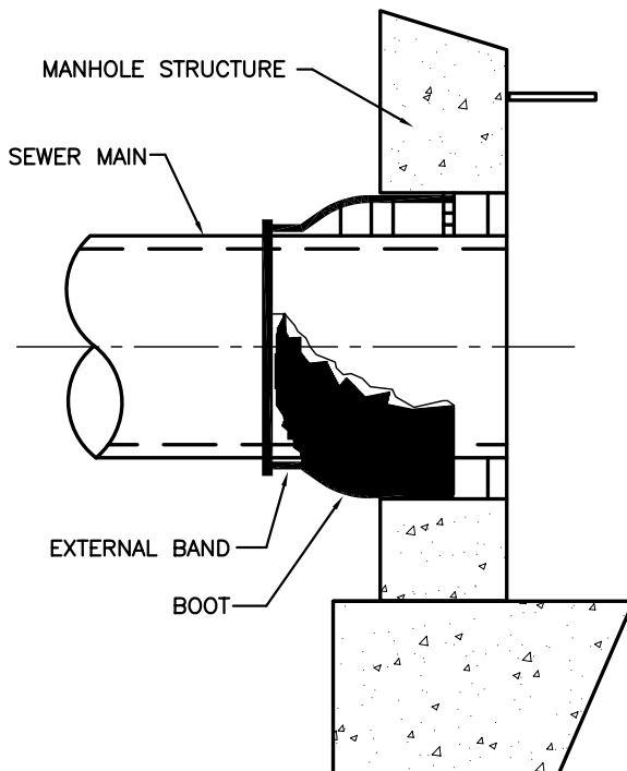
FLEXIBLE JOINT CONNECTION ASTM C-443
