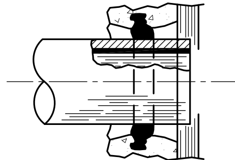
LOK GASKET DETAIL ASTM C-443
